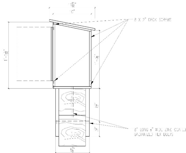
S2 FREE LIBRARY SIDE SECTION 3" = 1' - 0"
